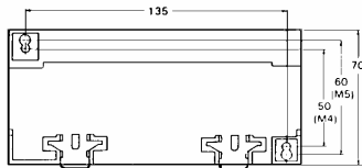
Rear View Showing Panel Mounting Holes
